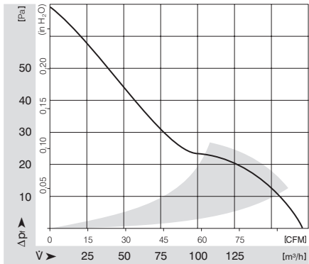
Characteristic: Pressure over air flow
