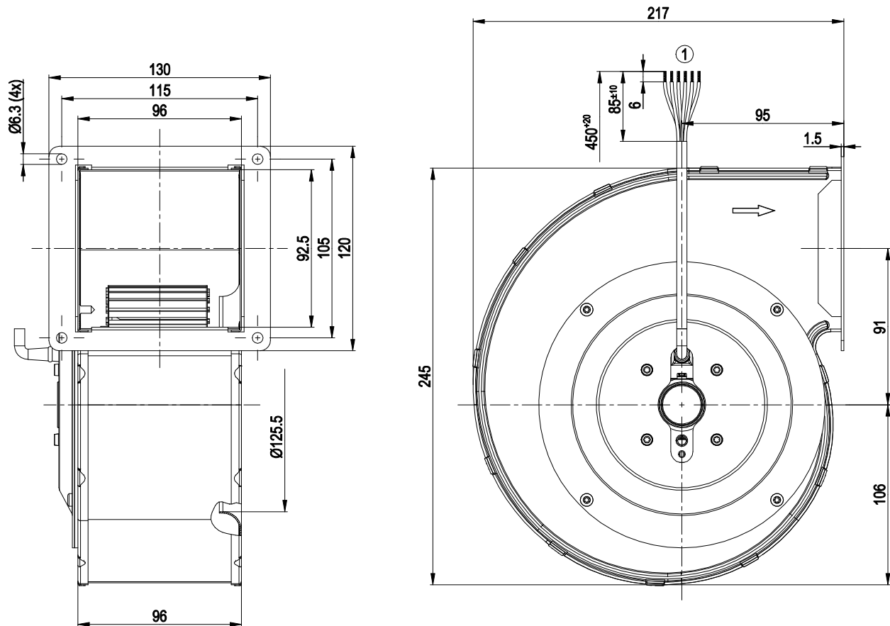
1 Cable XLPE/XLPO 6G 0.5 mm 2 , 6x crimped splices
