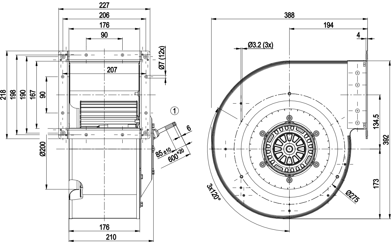
1 Cable silicone 6G 0.5 mm², 6x crimped splices
