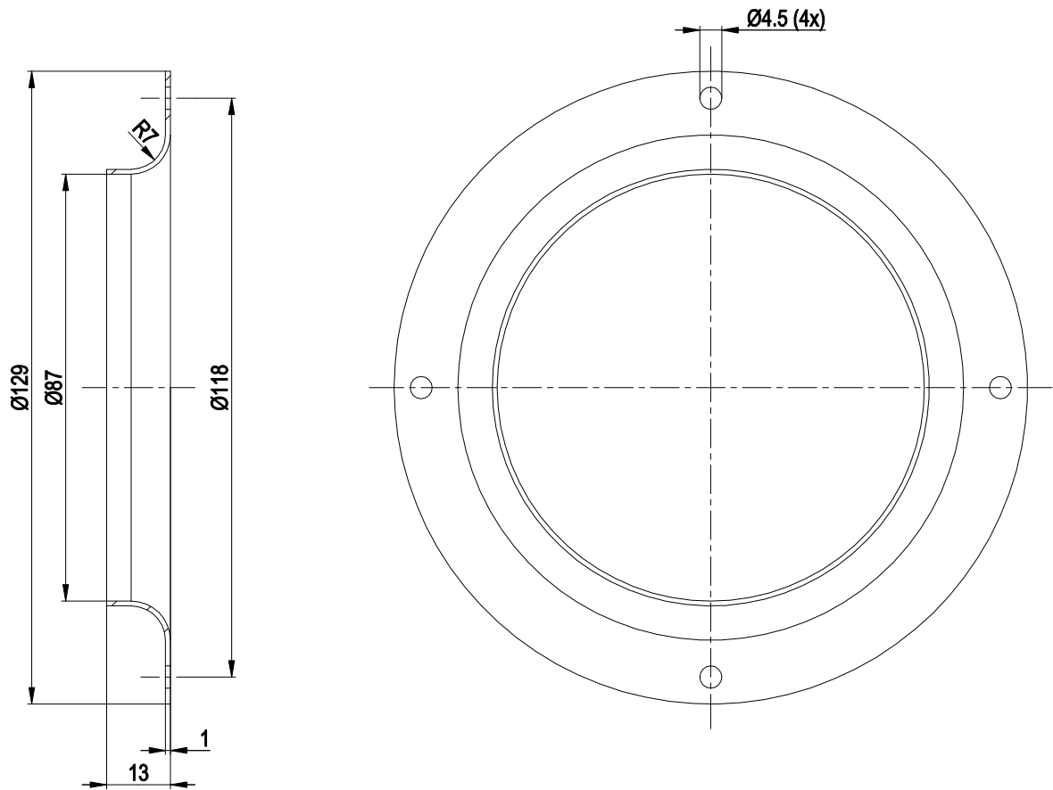
Inlet ring 09566-2-4013
