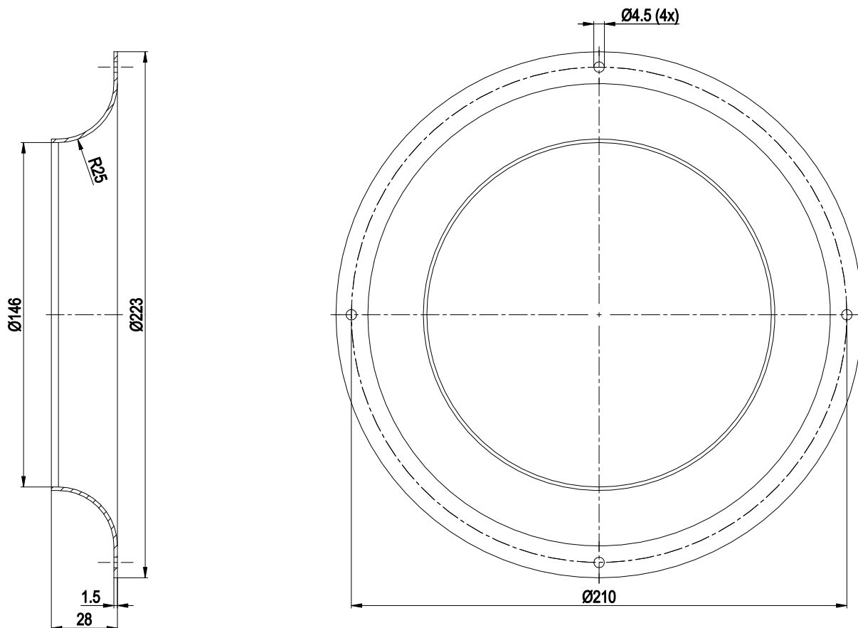
Inlet ring 96358-2-4013
