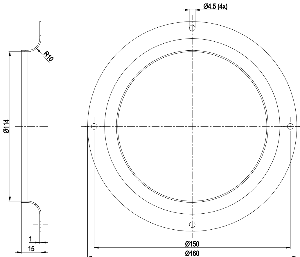
Inlet ring 09567-2-4013
