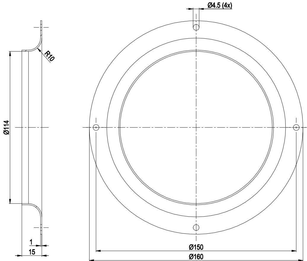
Inlet ring 09567-2-4013
