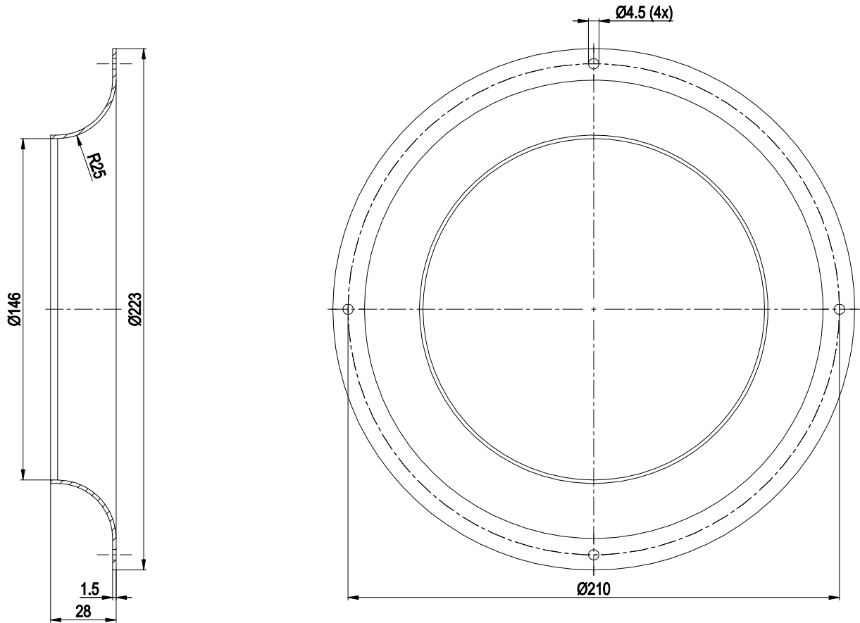
Inlet ring 96358-2-4013
