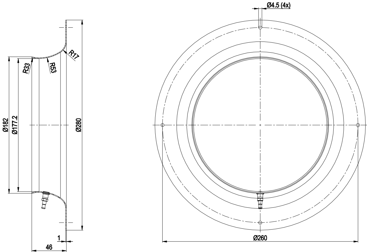
Inlet ring 28004-2-4013 with pressure tap (k-factor: 77)
