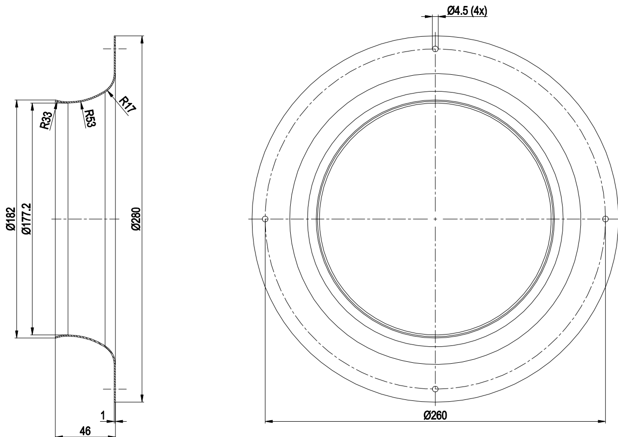
Inlet ring 28000-2-4013
