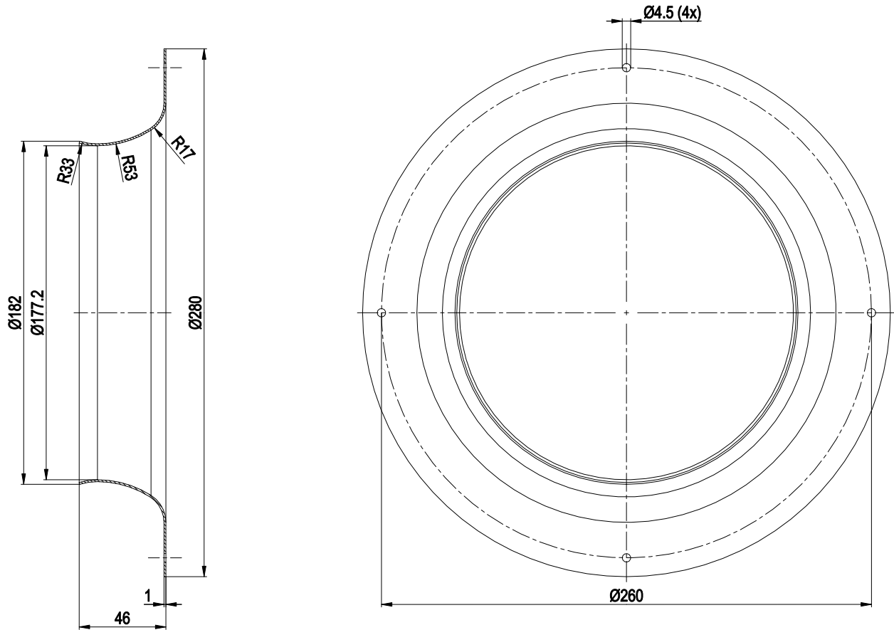
Inlet ring 28000-2-4013
