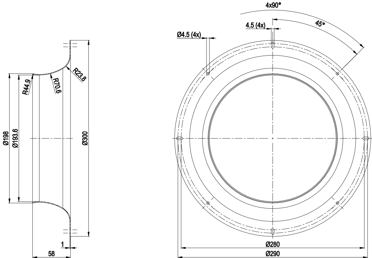
Inlet ring 31000-2-4013
