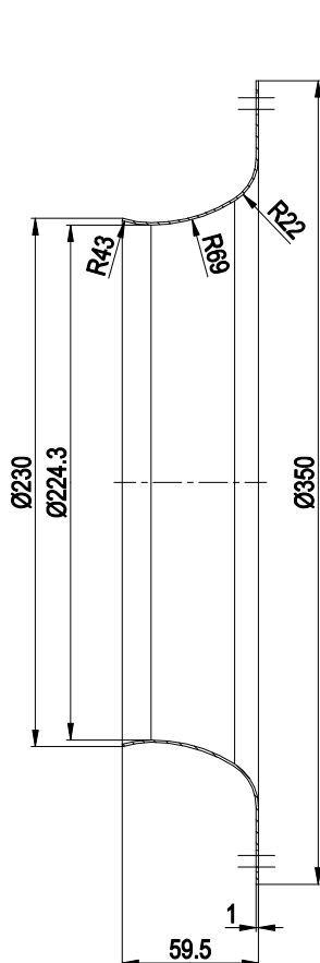
Inlet ring 35500-2-4013
