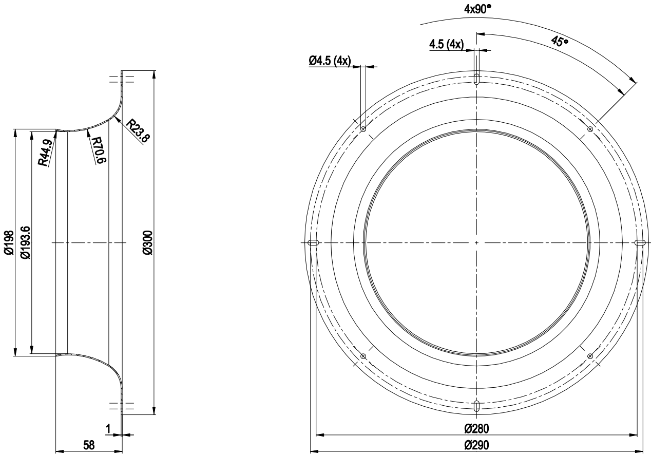
Inlet ring 31000-2-4013
