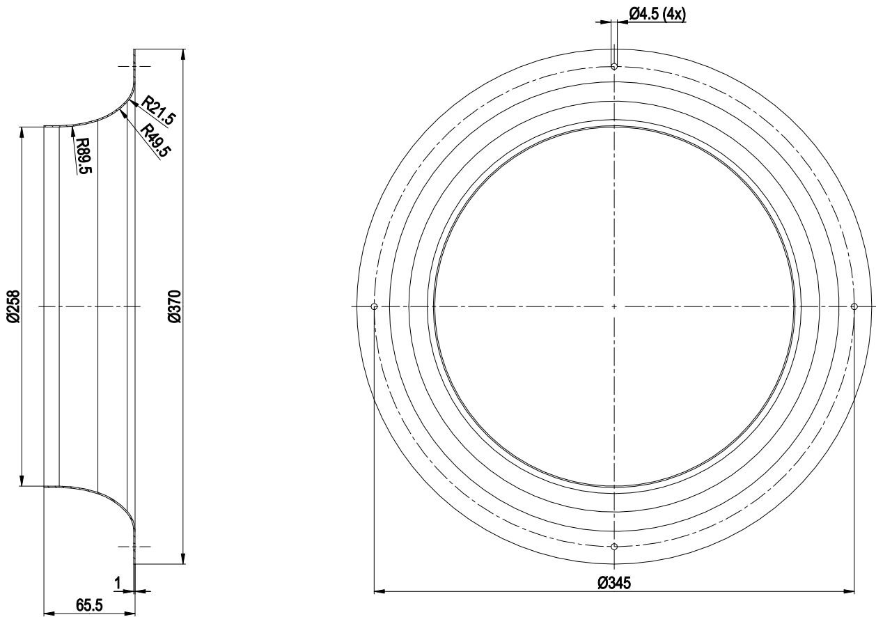
Inlet ring 54476-2-4013
