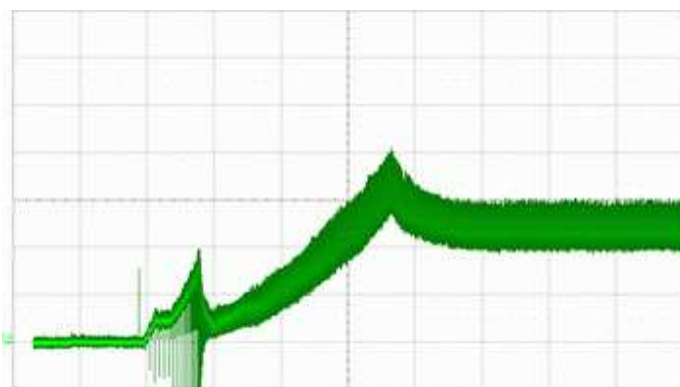
Start-up current @ 24 V ( I = 1\text{A/div} ; t = 2\text{s/div} )
