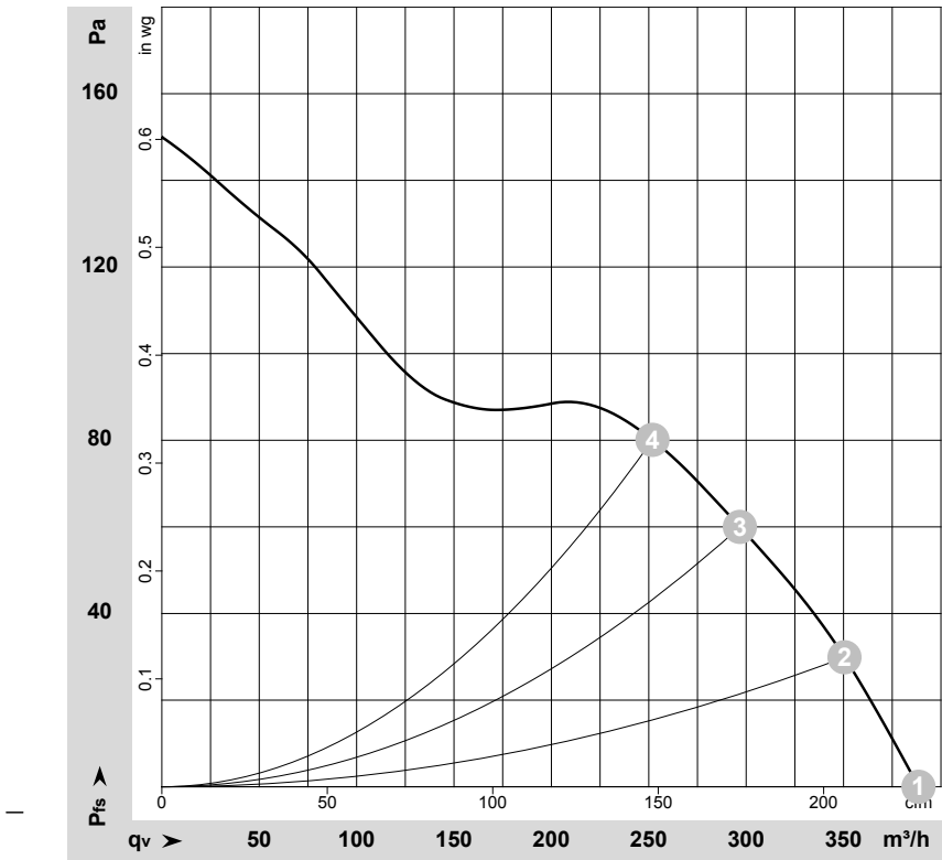
Curves: Air performance 60 Hz
