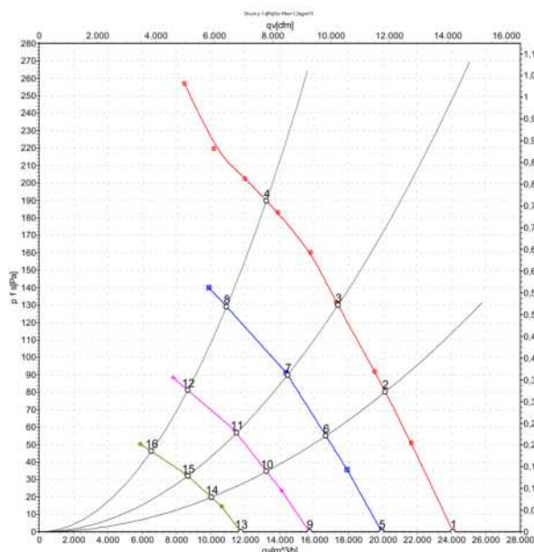
Charts: Air flow 50 Hz
