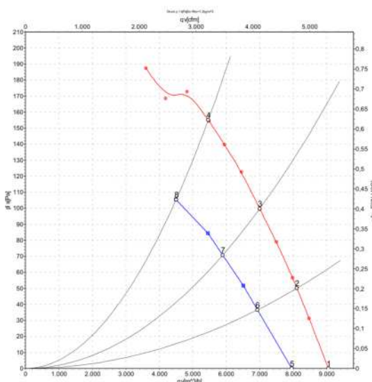
Curves: Air performance 50 Hz
