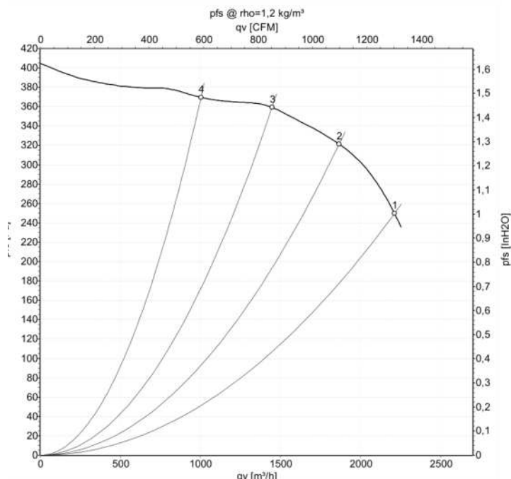
Charts: Air flow 50 Hz
