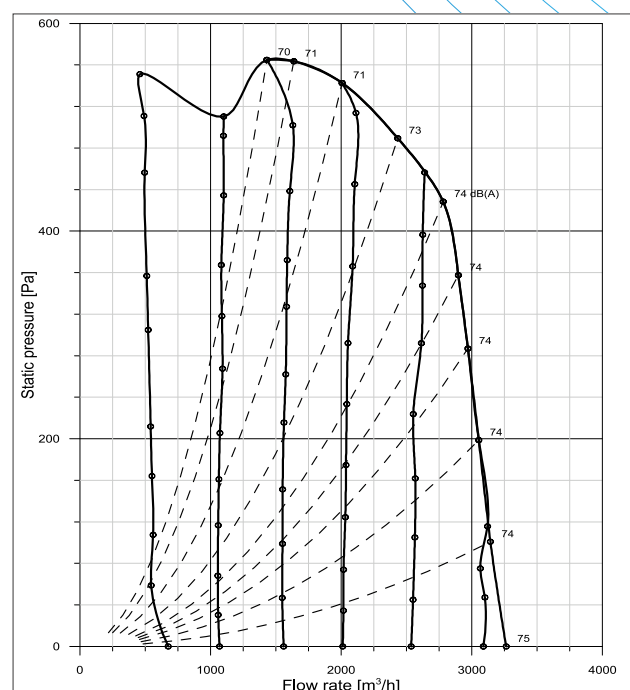
Constant Airflow Curve Graphic
