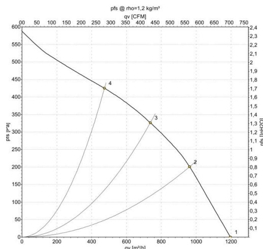
Charts: Air flow 50 Hz
