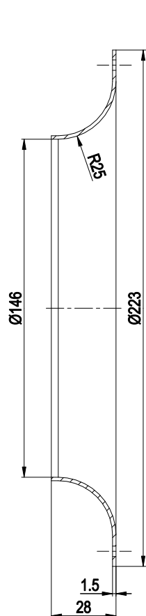
Inlet ring 96358-2-4013
