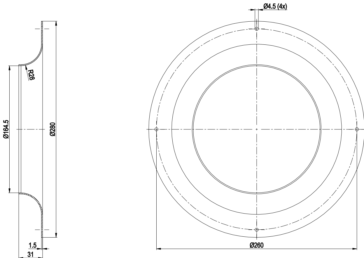
Inlet ring 96420-2-4013
