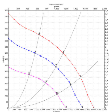
Curves: Air performance
