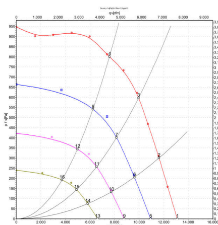
Curves: Air performance 50 Hz
