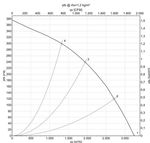
Curves: Air performance 50 Hz
