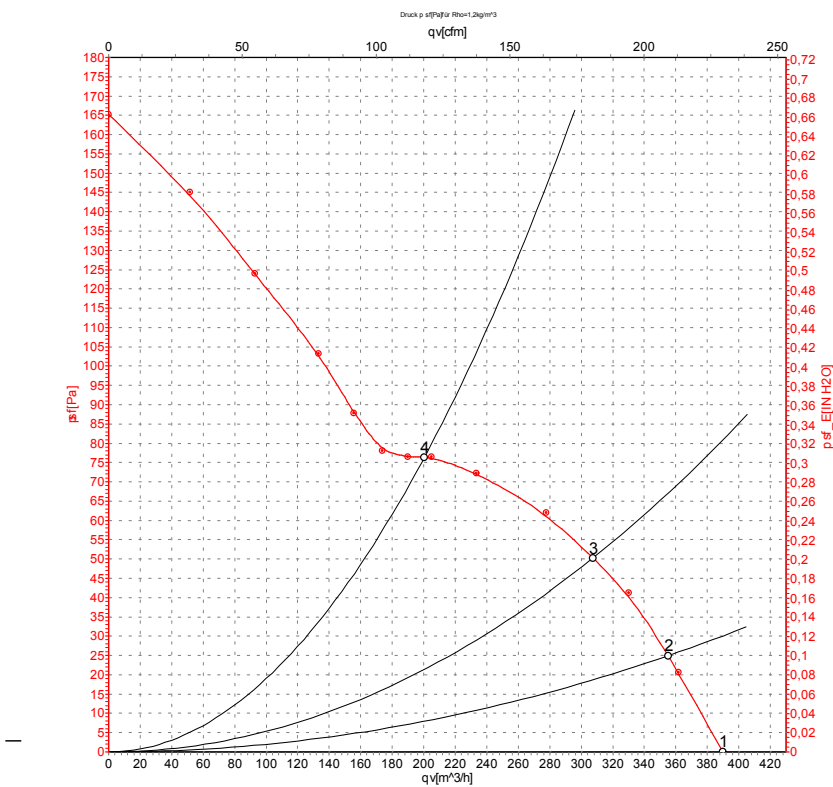
Charts: Air flow 60 Hz
